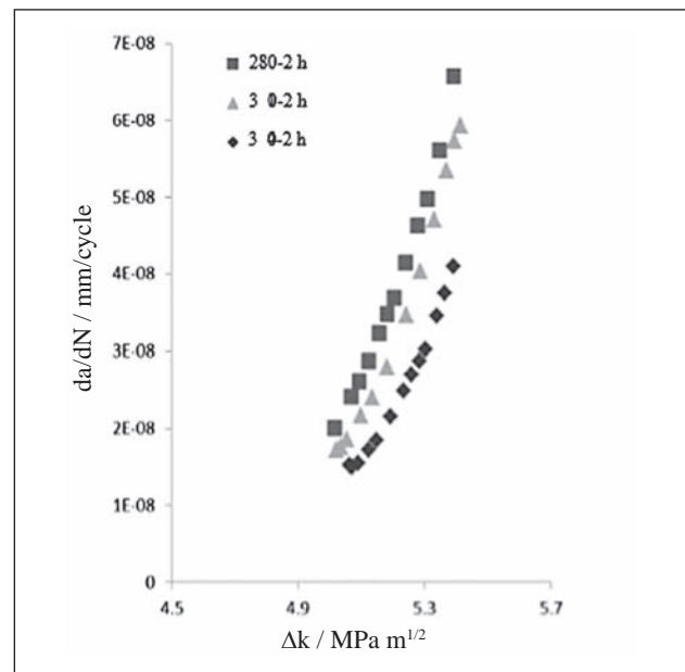
Figure 3 The fatigue crack propagation ( da/dN ) and stress intensity ( \Delta k ) of nodular cast iron in various temperatures holding time of 120 minutes
