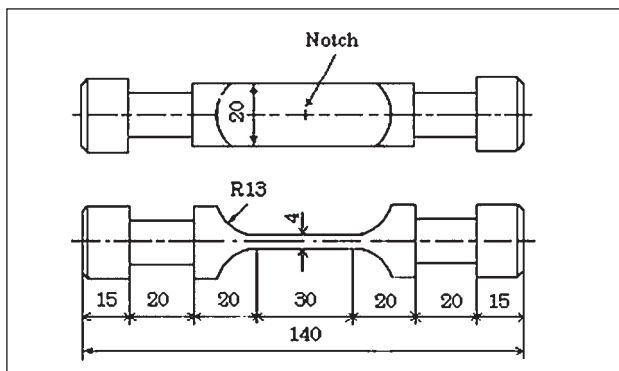
Figure 1 The specimen of the fatigue crack test [12]
