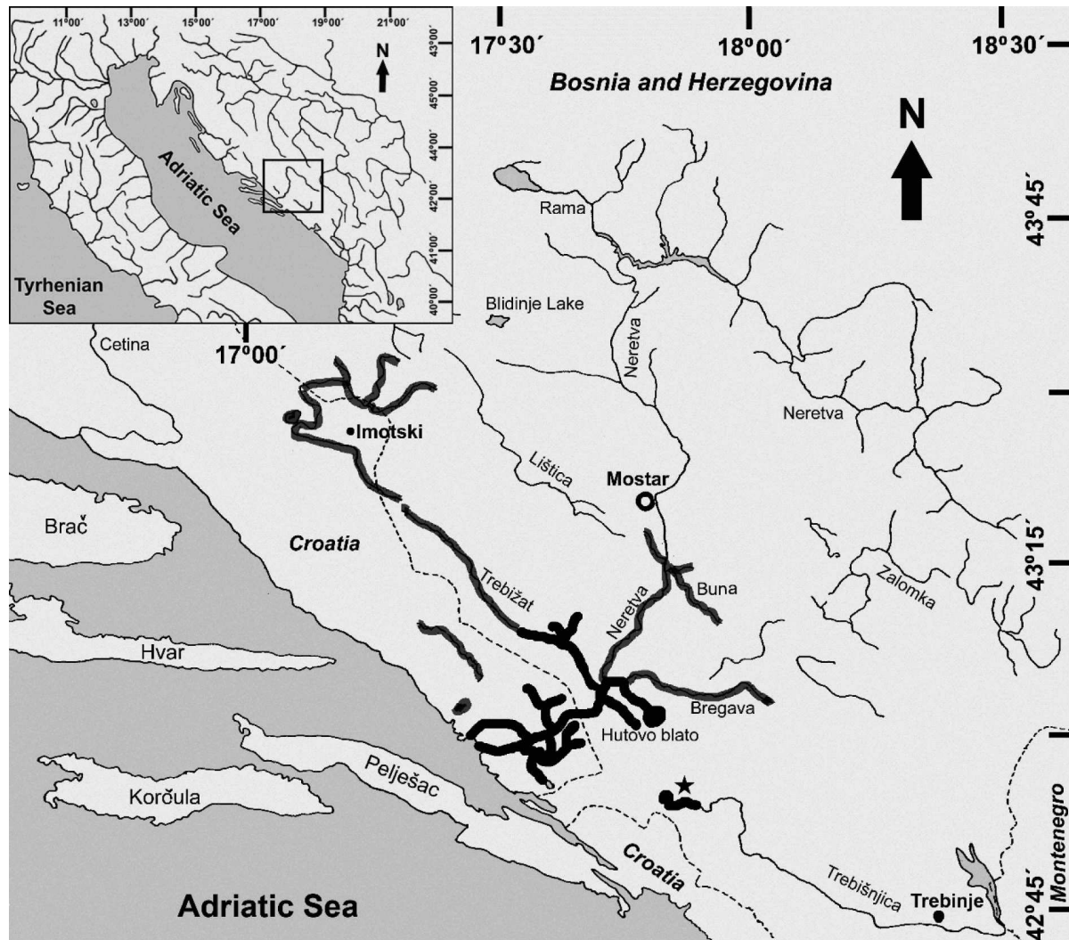
Fig 2. Distribution map of Neretva roach Rutilus basak (Heckel, 1843) (bold black lines) in the Adriatic drainage basin. The star indicates a new record in the Trebišnjica Channel above the Svitavsko accumulation of the Hutovo Blato wetland (Bosnia and Herzegovina).
