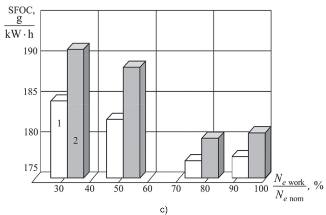
Figure 7 The Change in the Specific Effective Fuel Consumption of the SFOC of the Mitsubishi Marine Diesel Engine 7UEC60LS Depending on the Load for Various Degrees of Recirculation: a) EGR=4.7 %; b) EGR=9.8 %; c) EGR=14.6 %; d) EGR=18.8 %; 1 – operation without recirculation; 2 – operation with recirculation
