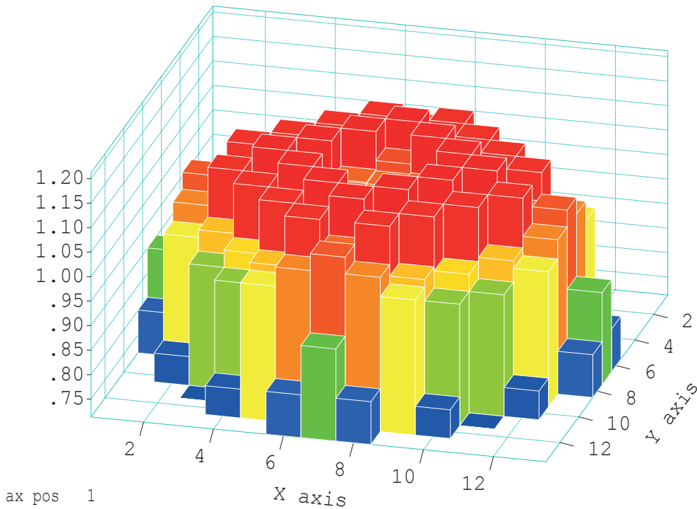
Figure 9: Relative power distribution at Bu = 13 \text{ GWd/tU}
