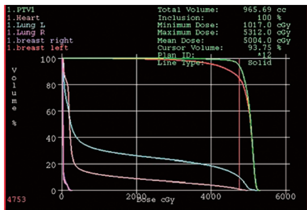
Figure 6. Dose Volume Histograms (DVH) for forward IMRT (left) and inverse IMRT (right)
