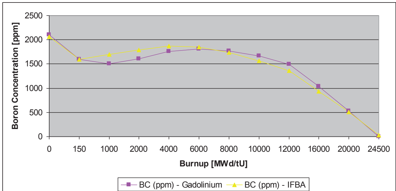
Figure 6: Stepwise critical Boron concentration for Gadolinium and IFBA based 24-month equilibrium cycles
