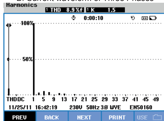
D. Harmonic Spectrum in A-Phase
