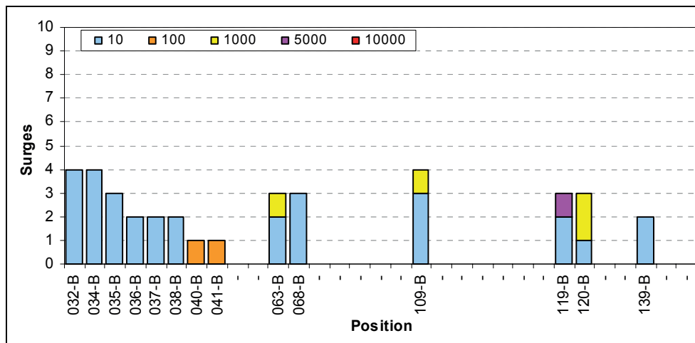
Figure 6-Review of LSA surges registered by Excourt II monitoring sensors in Phase L1 (B)
