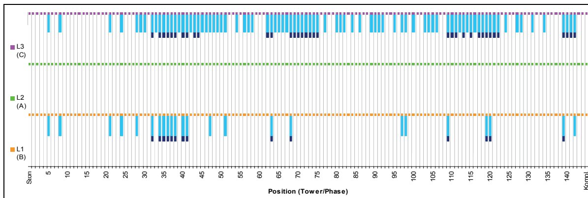
Figure 4-LSA arrangement along the line and installed Excourt II monitoring sensors (dark blue or black)
