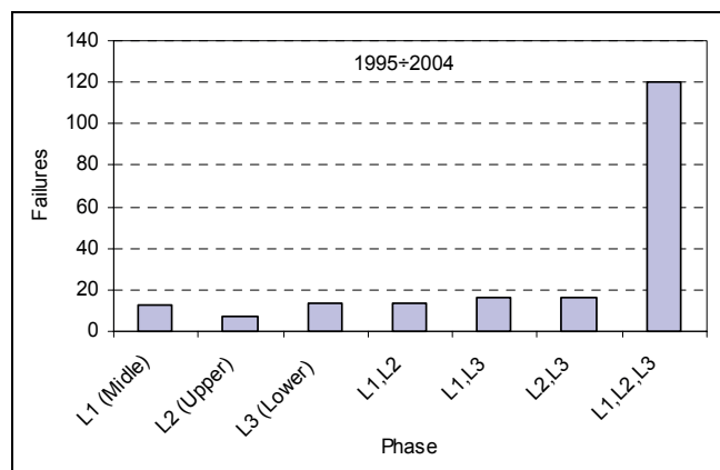
Figure 8- Review of events on line registered by distant relay protection
