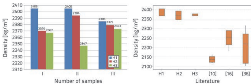
Figure 6. Density data
