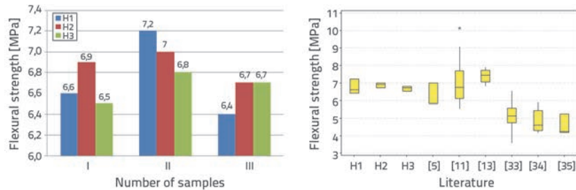
Figure 5. Flexural strength
