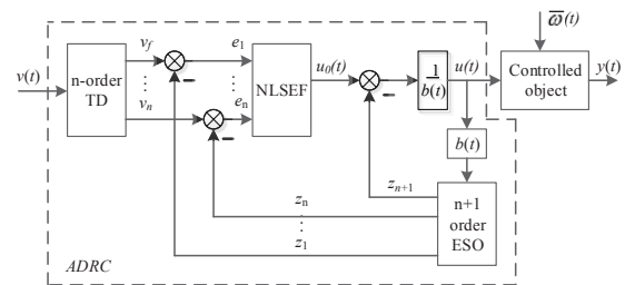
Fig. 3. The diagram of ADRC
