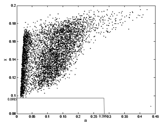
Fig. 9. The impedances seen by relay R_1 for faults in L_2 together with zone 1 setting of relay R_1
