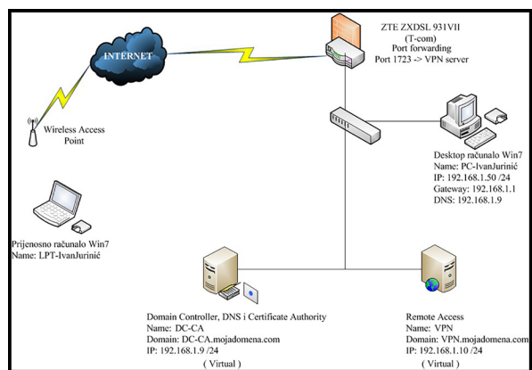
Figure 1 Network infrastructure
