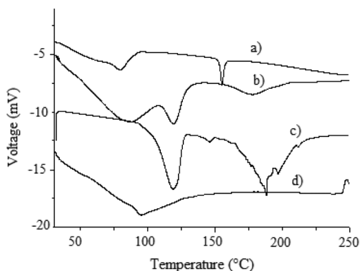
Fig. 5. DSC thermograms of: a) MR, b) physical mixture, c) MC and d) Amberlite® IRP 88.
