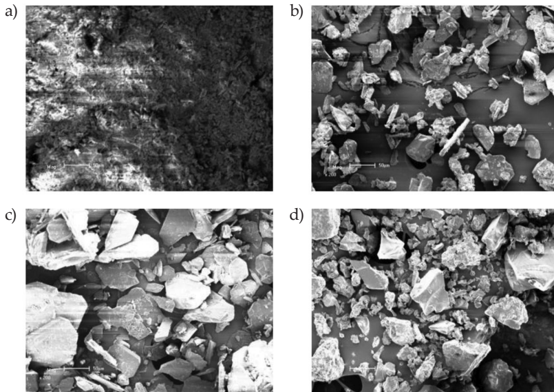
Fig. 7. Scanning electron micrographs of: a) MR, b) physical mixture, c) MC, d) Amberlite® IRP 88.
