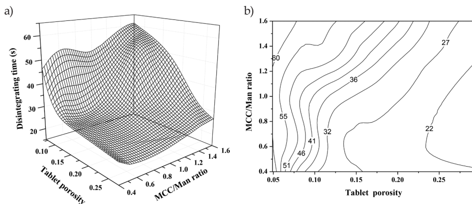
Fig. 8. Response surface and contour plots of disintegration time. MCC/Man ratio is ratio of microcrystalline cellulose and mannitol.
