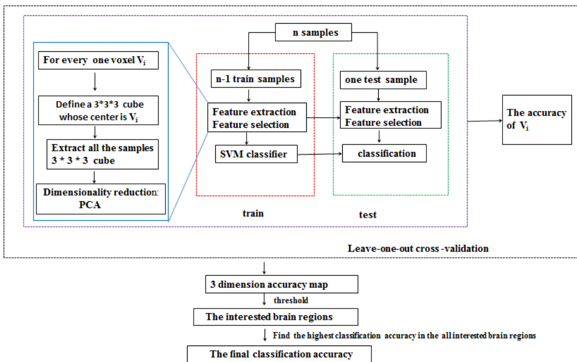
Figure1. The flow chart of classification. V_i : voxel i ; n was the number of patients; PCA: principal component analysis.
