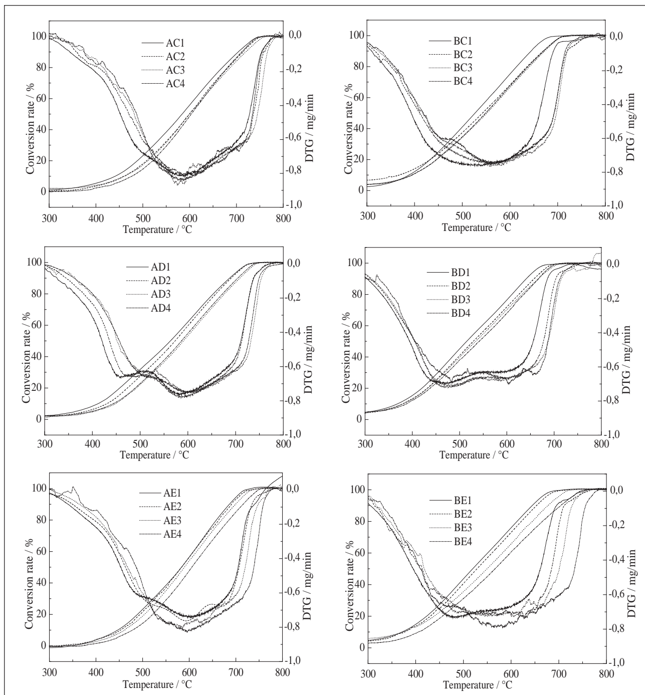
Figure 2 Co-combustion behavior of blends
