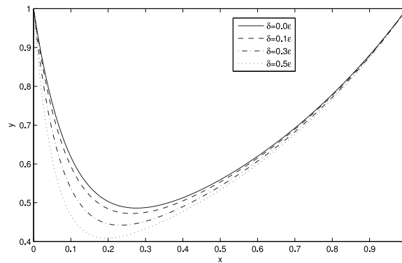
Figure 2: Left layer solution of Example 2 for \epsilon = 0.1 , N = 10^2 and different values of \delta
