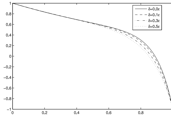
Figure 3: Right layer solution of Example 3 for \epsilon = 0.1 , N = 10^2 and different values of \delta
