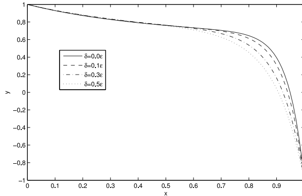
Figure 4: Right layer solution of Example 4 for \epsilon = 0.1, N = 10^2 and different values of \delta
