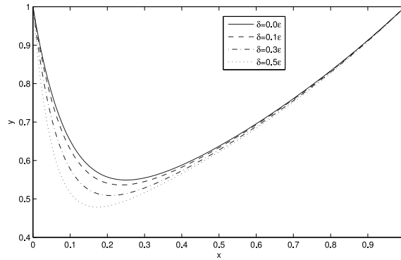
Figure 1: Left layer solution of Example 1 for \epsilon = 0.1 , N = 10^2 and different values of \delta
