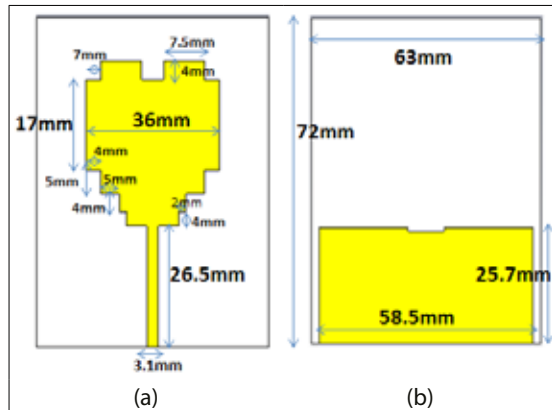
Fig. 1 configuration (a) Top view (b) Bottom view
