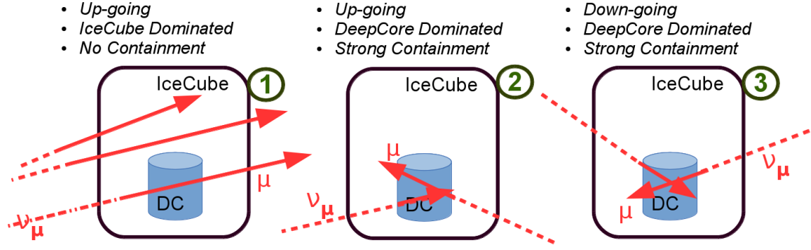
Figure 1: The three event selection strategies for the solar WIMP analysis. Most of the sensitivity for neutrino signals below 100 GeV comes from the DeepCore (DC) dominated low energy samples (2 and 3). During the austral summer (when the Sun is a source of downgoing neutrinos), the very large muon background forces us to use the outer detector as a Veto (see Fig. 2) and consequently there is only a DeepCore dominated-low energy sample (3). This approach is similar to that of earlier IceCube analyses such as [7].
