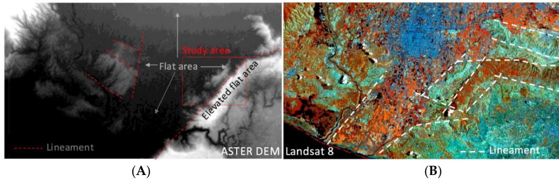
Figure 12. Lineament identification, (A) Lineament interpretation based on ASTER DEM; (B) Lineament interpretation based on the Landsat 8.
