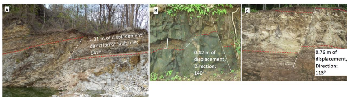
Figure 17. (A) Fault displacement in the outcrop 17 segment 3; (B) displacement in outcrop 26 segment 1; (C) Fault displacement in outcrop 56.
