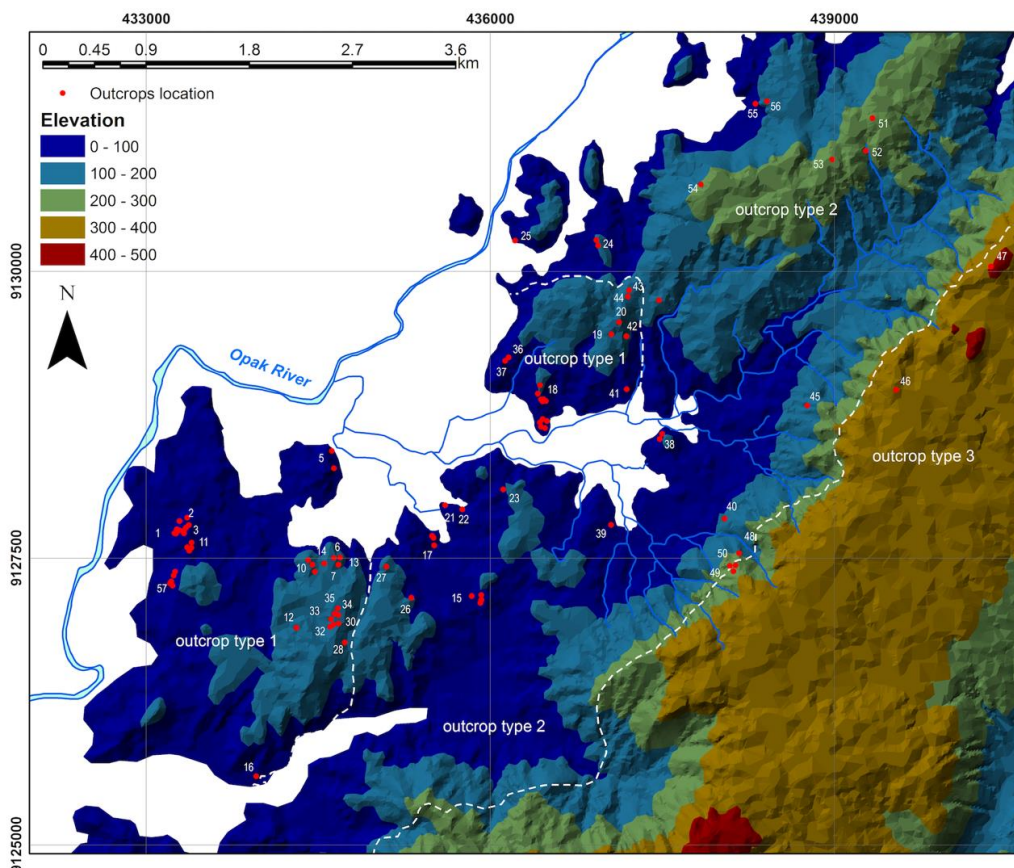
Figure 16. Outcrops classification.
