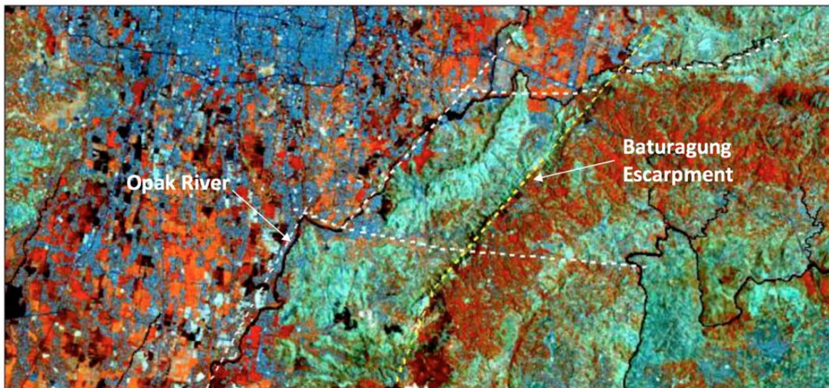
Figure 13. Opak River and Baturagung Escarpment lineament.
