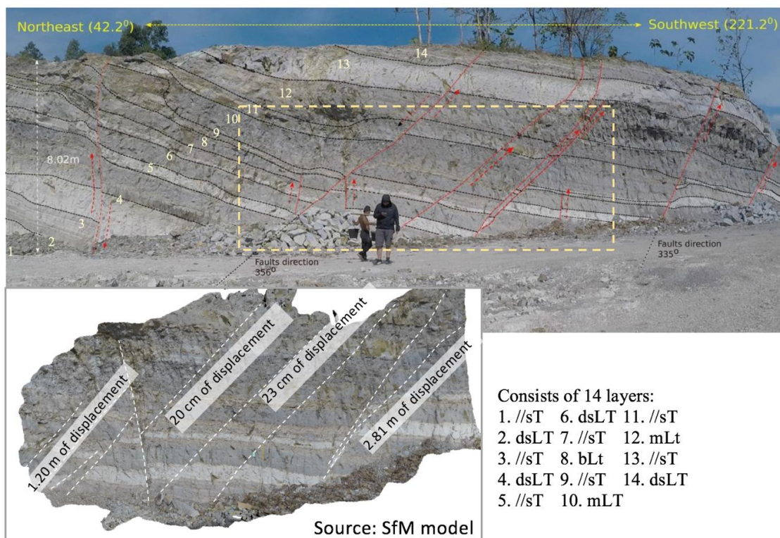
Figure 18. The outcrop 73.
