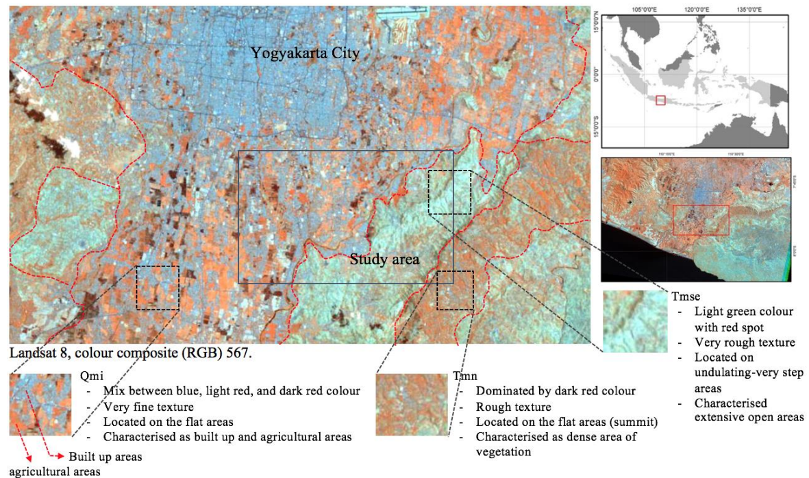
Figure 9. The lithological characteristics based on the Landsat 8 image, colour composite (RGB) 567.
