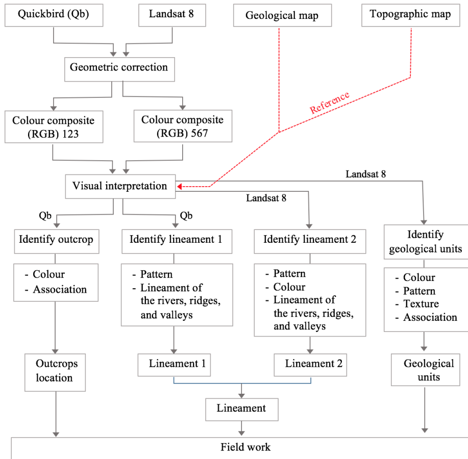
Figure 6. Pre-fieldwork framework.
