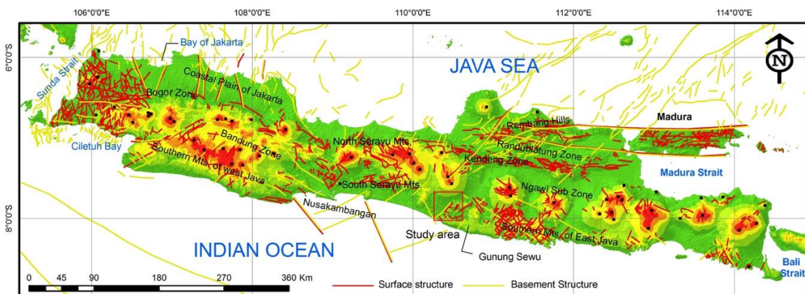
Figure 3. Fault configuration of Java (modified from [4]).
