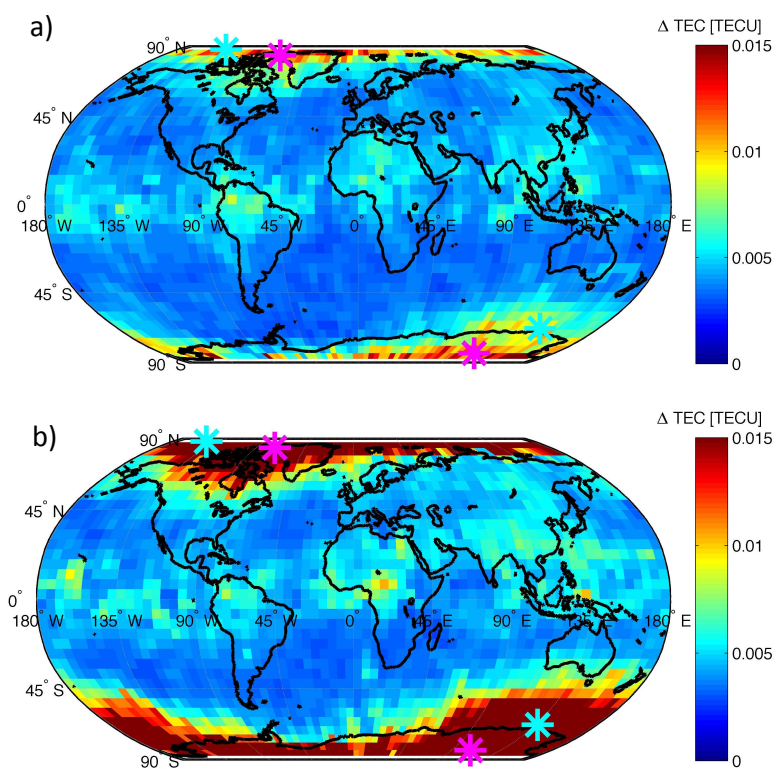
Figure 4. a) Global map of \Delta TEC during September 2008 (solar minimum). b) Global map of \Delta TEC during September 2013 (solar maximum). The geomagnetic (magnetic) poles are indicated by the magenta (cyan) star symbols respectively.
