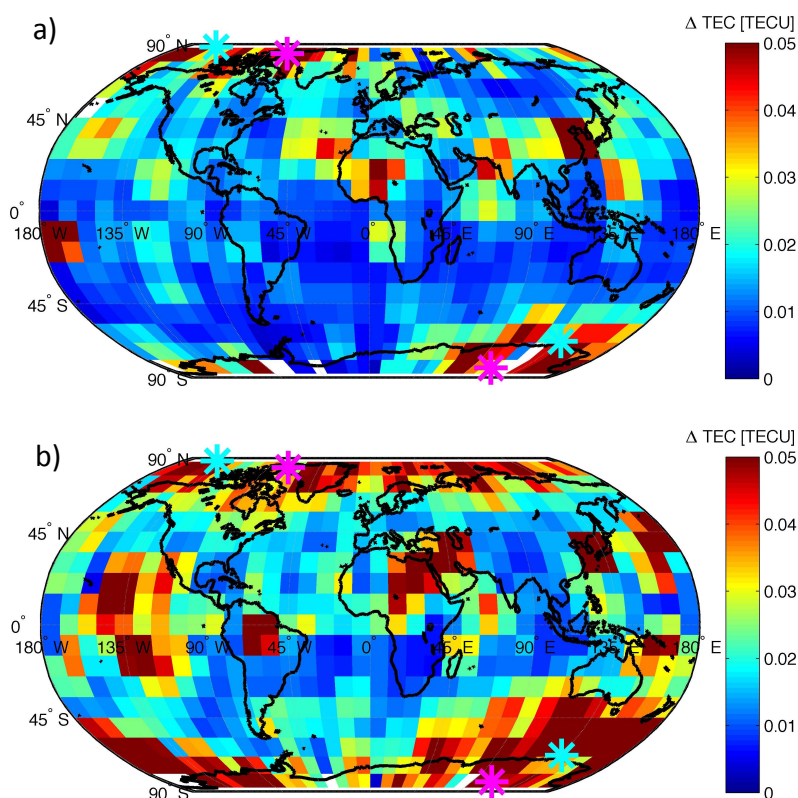
Figure 7. a) Global map of \Delta\text{TEC} (tangent points at h=200\text{--}300 km) during the quiet phase, and b) during the storm phase of the geomagnetic storm of 15 July 2012. The arithmetic mean is applied to the values of the binned cells ( 10^\circ \times 10^\circ in latitude and longitude). The geomagnetic (magnetic) poles are indicated by the magenta (cyan) star symbols respectively.
