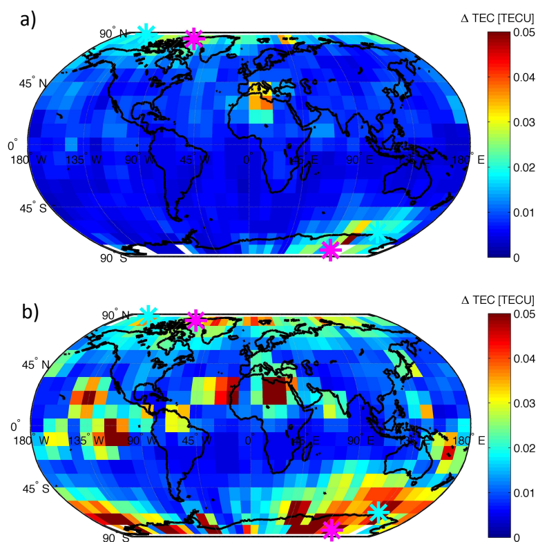
Figure 6. a) Global map of \Delta\text{TEC} (tangent points at h=400\text{-}500 km) during the quiet phase, and b) during the storm phase of the geomagnetic storm of 15 July 2012. The arithmetic mean is applied to the values of the binned cells ( 10^\circ \times 10^\circ in latitude and longitude). The geomagnetic (magnetic) poles are indicated by the magenta (cyan) star symbols respectively.
