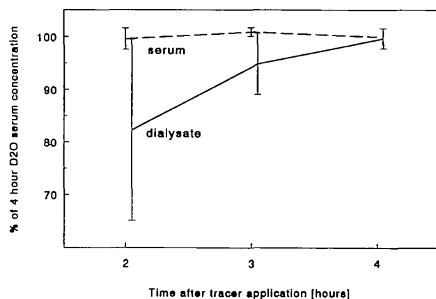
Fig. 1. Equilibration of D 2 O in serum (---) and dialysate (—) in peritoneal dialysis patients 2, 3 and 4 h after tracer application (mean ± SD).
