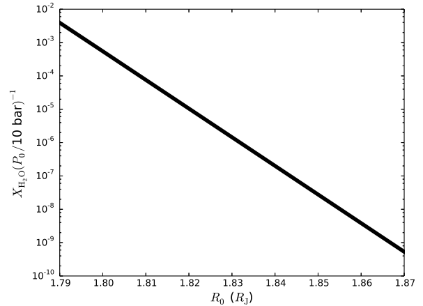
Figure 7. Inferred water abundances, obtained from best fits to the measured WFC3 transmission spectrum of WASP-12b from Kreidberg et al. (2015), versus the assumed value of the reference transit radius.
