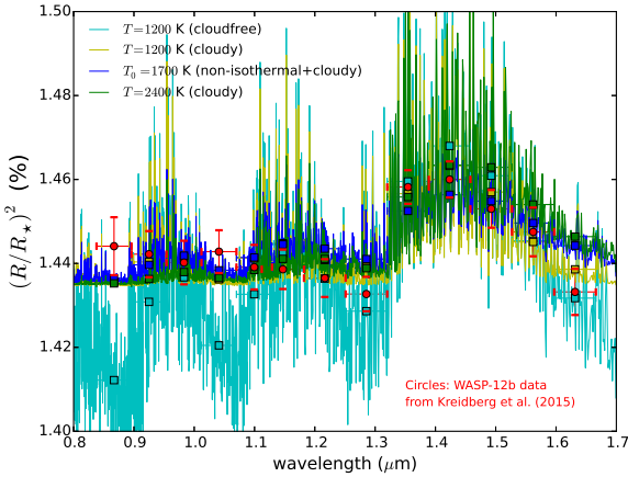
Figure 2. Examples of model transmission spectra with different temperatures, cloud opacities and a finite temperature gradient. The water volume mixing ratio is set to 10^{-3} for illustration. See Table 1 and text for the parameter values assumed for these models.
