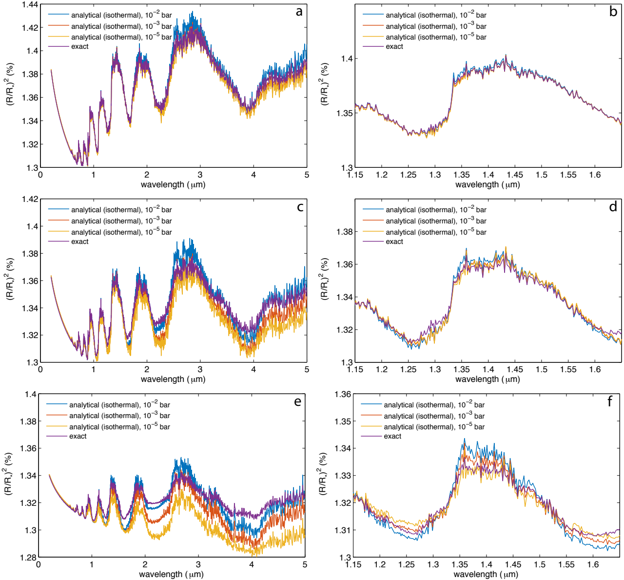
Figure 4. Comparing our full numerical calculations of the transmission spectrum of an isothermal atmosphere to those computed using our isothermal, isobaric analytical formula. The first, second and third rows are for T = 1500 K, T = 1000 K and T = 500 K, respectively. The left and right columns are for JWST-NIRSpec and HST-WFC3 wavelength coverage, respectively. We used a spectral resolution \sim 0.1 \text{ cm}^{-1} for the opacity function and then binned the model down to a resolution \sim 10 \text{ cm}^{-1} . These calculations demonstrate that WFC3 transmission spectra may be approximated as being isobaric (constant pressure) in some instances.
