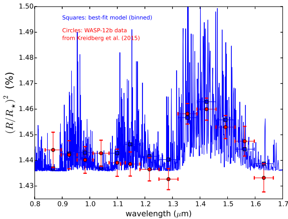
Figure 6. Best-fit model using our analytical isothermal, isobaric formula to the measured WFC3 transmission spectrum of WASP-12b from Kreidberg et al. (2015).
