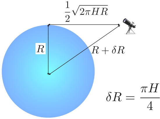
Figure 1. Schematic illustrating the transit geometry for an isothermal atmosphere, which has an effective chord length of \sqrt{2\pi HR} corresponding to the transit radius (Fortney 2005). This works out to \delta R = \pi H/4 , which is a change in pressure of a factor of \exp(\pi/4) \approx 2.19 across the transit chord.
