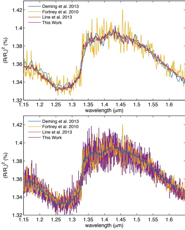
Figure 3. Benchmarking our full numerical calculation of the transmission spectrum of HD 209458b (see text for details of input parameters) to those of Fortney et al., Deming et al., and Line et al. We used a spectral resolution of \sim 0.1 \text{ cm}^{-1} for the opacity function to compute the model transmission spectrum. In the top and bottom panels, we then binned down the model to resolutions of \sim 10 \text{ cm}^{-1} and \sim 1 \text{ cm}^{-1} , respectively, to illustrate that minor discrepancies result from adopting different spectral resolutions for the water opacity. (Discrepancies may also arise from the use of different spectroscopic line lists to construct the opacity function.)
