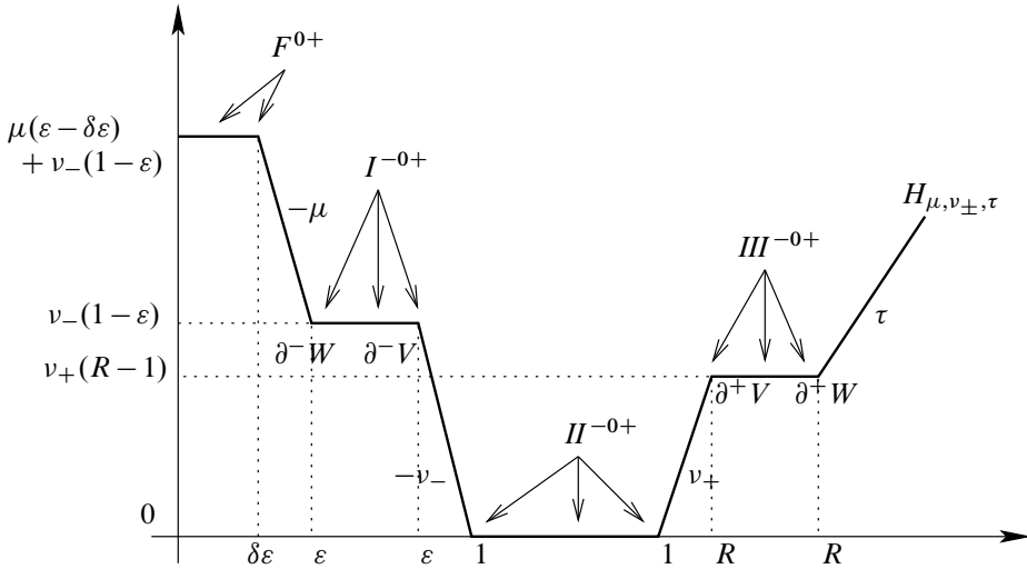
Figure 18: Hamiltonian adapted to the construction of the transfer map \text{SH}_*^Q(W) \rightarrow \text{SH}_*^Q(V)
