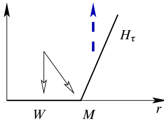
Figure 1: Symplectic homology of a domain
