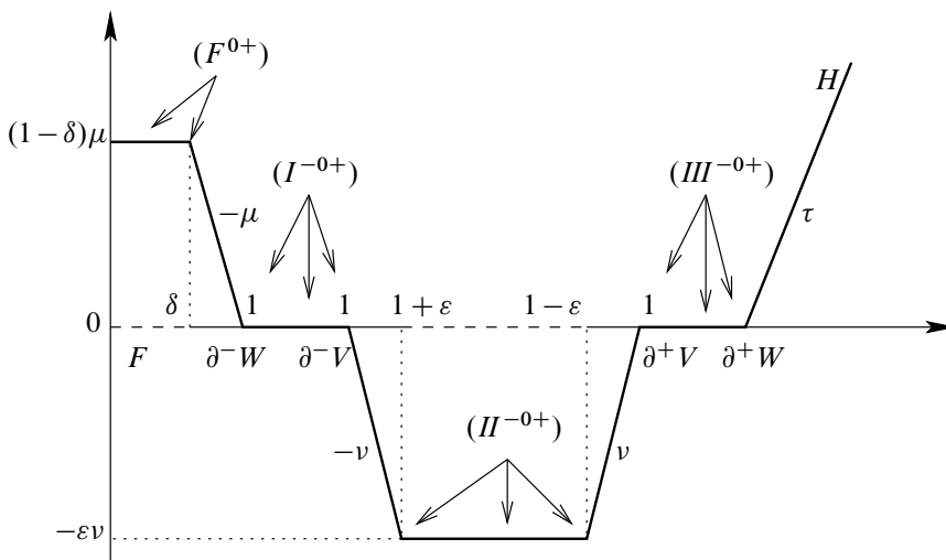
Figure 14: Hamiltonian in \mathcal{H}(W, V; F)
