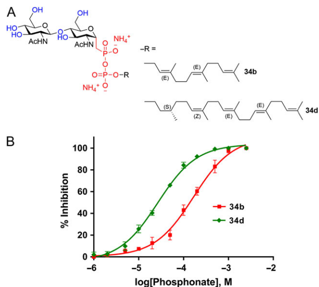
Fig. 5. (A) Structure of the LLO inhibitors synthesized ( 34b ) farnesyl-PP-C-chitobiose, C 15 ; ( 34d ) (S)-farnesylCitronellol-PP-C-chitobiose, C 25 . (B) Kinetic analysis of synthetic LLO inhibitors. Glycosylation experiments were performed with 20 nM TbSTT3A protein, 10 \mu M peptide P11, 10 mM MnCl 2 , 150 mM NaCl, 20 mM Hepes pH 7.5, 0.035% DDM and 0.007% CHS. Samples were incubated with LLO competitive inhibitors (1–2500 \mu M) for 5 min before adding 15 \mu M of farnesyl-PP-chitobiose, 1b . Data points reflect the mean of three separate measurements. Error bars indicate standard deviations. Data were fitted by nonlinear regression using PRISM software. This figure is available in black and white in print and in color at Glycobiology online.
