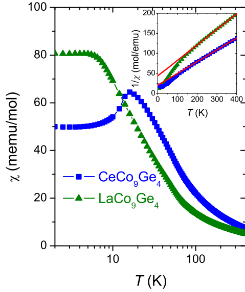
Figure 2. The magnetic DC susceptibility \chi versus T of \text{CeCo}_9\text{Ge}_4 and \text{LaCo}_9\text{Ge}_4 measured in an external field of 0.5 T. Inset: Inverse magnetic DC susceptibility 1/\chi versus T of \text{CeCo}_9\text{Ge}_4 (squares) and \text{LaCo}_9\text{Ge}_4 (triangles). The solid lines are fits based on a modified Curie-Weiss type law, \chi(T) = C/(T - \Theta_{\text{CW}}) + \chi_0 .
