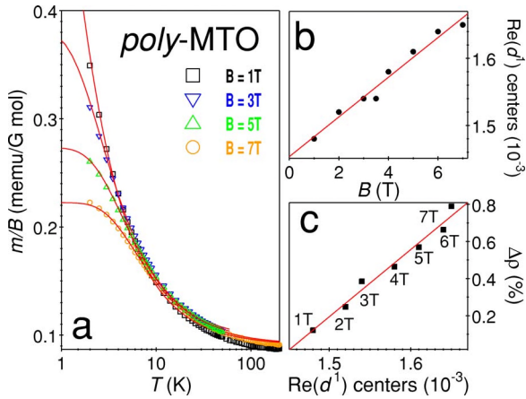
FIG. 10. (Color online) (a) m/B of poly -MTO in several external magnetic fields. The solid lines are Brillouin fits for a \text{Re}(d^1) configuration. (b) The amount of \text{Re}(d^1) centers deduced from the fits vs B . (c) Percentage increase of the resistivity with magnetic field vs the amount of \text{Re}(d^1) centers.
