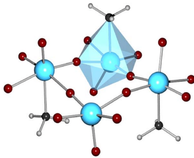
FIG. 3. (Color online) Top: The IR spectrum of poly -MTO exhibits an asymmetric ( 910\text{ cm}^{-1} ) and a symmetric ( 940\text{ cm}^{-1} ) Re—O stretching mode which clearly deviate from the corresponding values in the monomer MTO [ \nu_{as}(\text{ReO}_3) : 955\text{ cm}^{-1} ; \nu_s(\text{ReO}_3) : 1000\text{ cm}^{-1} ]. Bottom: DFT optimized structural model I of poly -MTO (see also Fig. 15).
