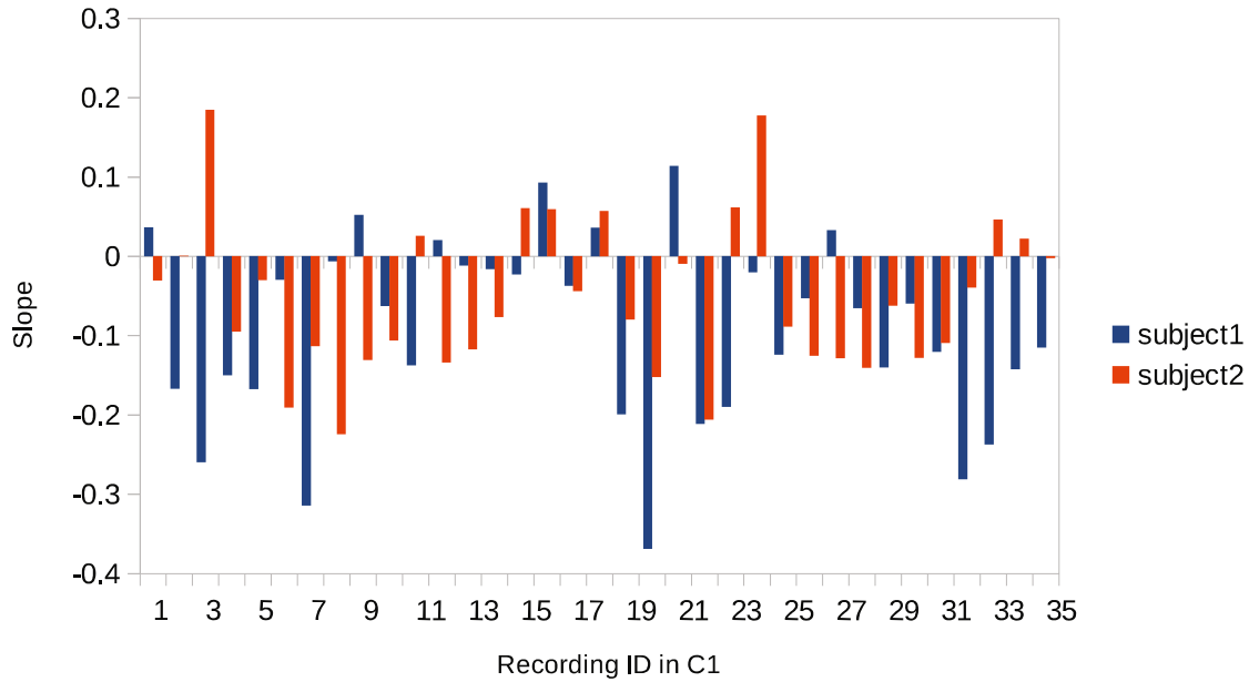
Fig. 2. Slope of RMSE sequences of 70 Chinese subjects from 35 recordings. In each recording, there are two subjects as denoted with blue and red bars, respectively. (Color figure online)
