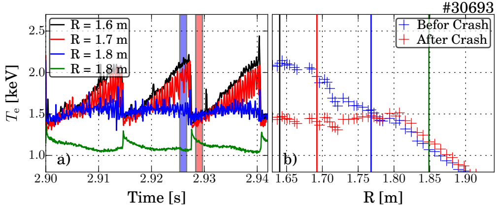
Figure 2.10.: In a) the time evolution of the temperatures during sawteeth at different radial positions can be seen. The eponymous sawtooth structure is clearly visible in the central channels. In b) the temperature profiles close before and after a sawtooth crash are shown. The figure is adapted from [19].
