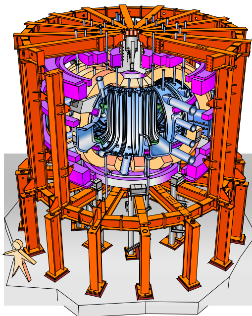
Figure 3.1.: Sketch of ASDEX Upgrade, with the support structure in orange, the poloidal field coils in magenta, the copper-colored toroidal field coils and the vacuum vessel with multiple diagnostic- and heating-ports in silver.
