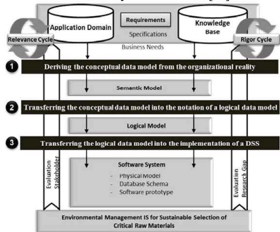
Figure 2. Applied conceptual data modeling procedure
