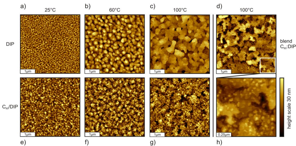
Figure 2. (upper row) AFM images of DIP films (50 nm) on PEDOT:PSS/ITO, evaporated at substrate temperatures of a) 25 °C b) 60 °C and c) 100 °C. (lower row) C_{60} (80 nm) on DIP (50 nm)/ PEDOT:PSS/ITO, with DIP evaporated at the same substrate temperatures as in the upper row. d) AFM image of C_{60} :DIP blend (mixing ratio 1:1, 50 nm)/ DIP (5 nm) on PEDOT:PSS/ITO evaporated at substrate temperature of 100 °C with magnification in h).
