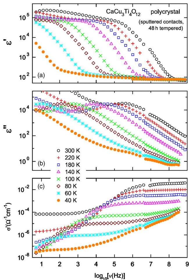
FIG. 2. (Color online) \epsilon'(\nu) (a), \epsilon''(\nu) (b), and \sigma'(\nu) (c) of polycrystalline CCTO (tempered 48 h) with sputtered gold contacts at various temperatures.
