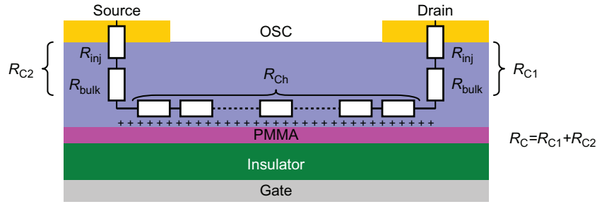
Figure 2. Schematic profile of a transistor channel with the contact resistance R_C (consisting of interface resistances R_{inj} and bulk resistances R_{bulk} ) and the channel resistance R_{ch} .
