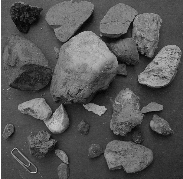
Figure 7. Sharp-edged fractured cobbles from the upper part of the intrusion and the uplifted beds.
