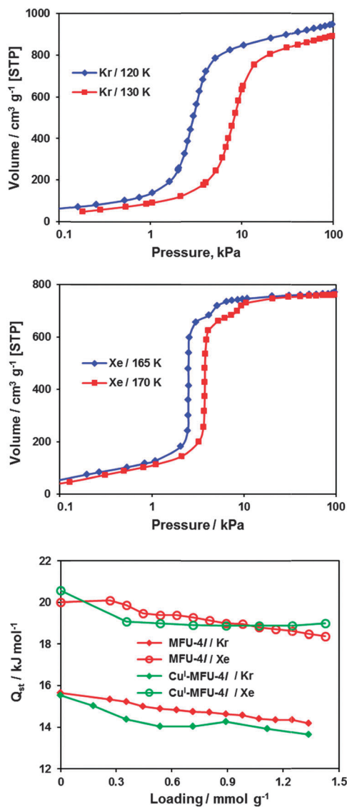
Fig. 3 Saturation adsorption isotherms for Kr (top) and Xe (middle) in \text{Cu}^{\text{I}} -MFU-4l in semilogarithmic scale, and dependencies of the isosteric heats of adsorption on loading for Kr and Xe in \text{Cu}^{\text{I}} -MFU-4l in comparison to MFU-4l 8 (bottom).
