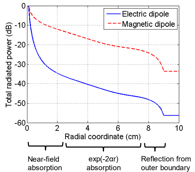
Fig. 1. Total radiated power as a function of the radial coordinate, for an elementary source implanted in the centre of a lossy host medium.
