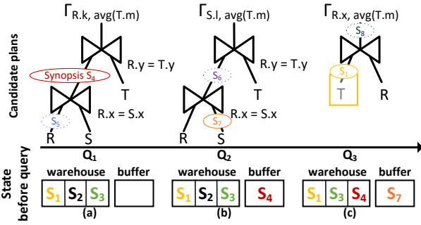
Fig. 2: Example execution of Taster. The dotted ellipses depict prospective synopses, the normal-line ellipses depict chosen synopses. Yellow boxes are used to denote reuse of existing synopses. \Gamma_{group,aggr} denotes aggregation operator with group grouping attributes and aggr aggregation function.
