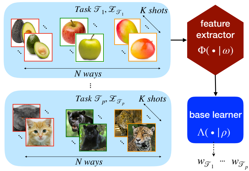
Figure 1. Base-learning of the task-specific parameters w_{\mathcal{T}_i} over p tasks following steps 3 to 6 of Algorithm 3.
