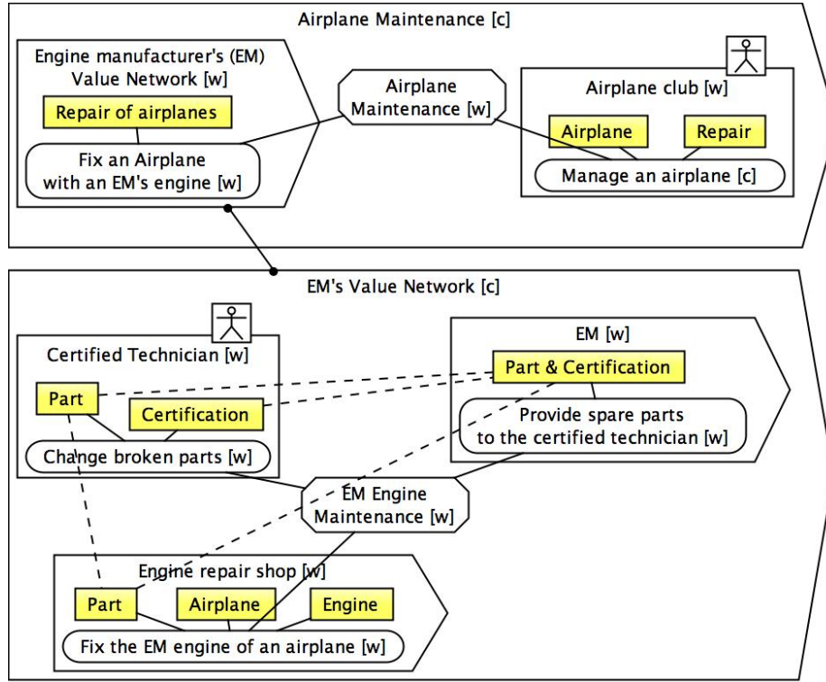
Fig. 5. Information Properties
