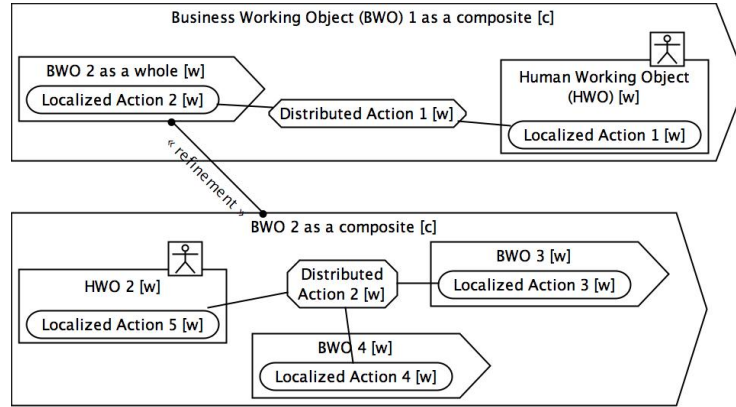
Fig. 1. Service System's Graphical Notation
