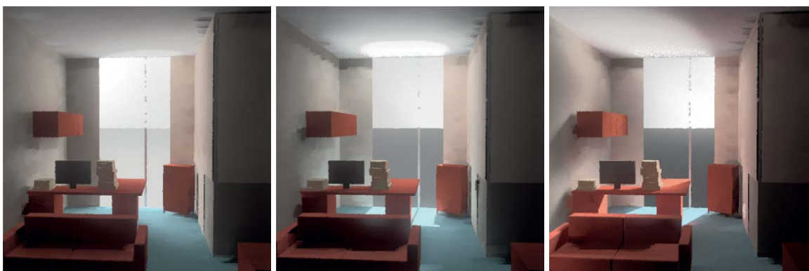
Simulated daylighting distribution in an office room through a Laser Cut Panel (LCP) at noon, 3PM and 5PM on Spring equinox.
