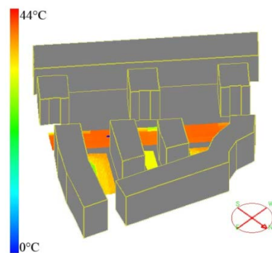
Figure 2: A snapshot of the road surface temperature of Rue des Maraîchers in Geneva (by G. Upadhyay)
