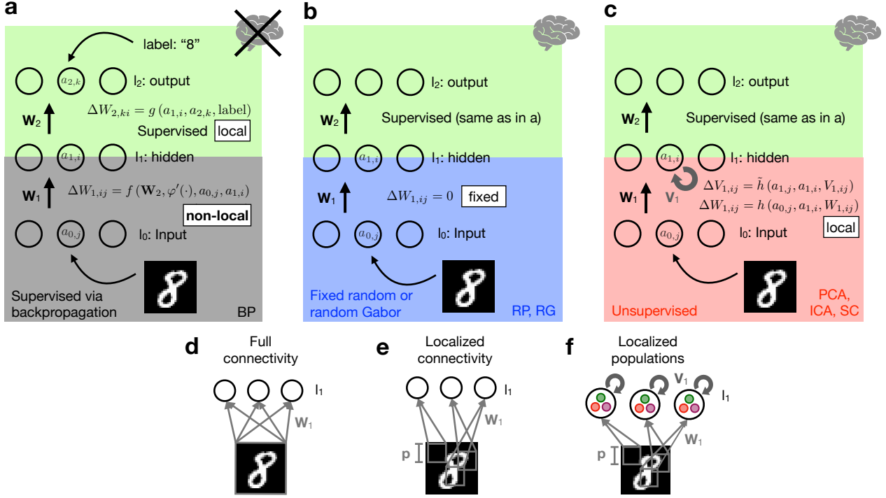
Figure 1: The proposed network model has one hidden layer ( l_1 ) and one readout layer ( l_2 ) of nonlinear units (nonlinearity \varphi(\cdot) ). Respective neural activations (e.g. a_{0,j} ) and update rules (e.g. \Delta W_{1,ij} ) are added. ( f(\cdot) , g(\cdot) , h(\cdot) & \tilde{h}(\cdot) are (non-)local plasticity functions, i.e. using only variables (not) available at the synapse for the respective update. a Training with backpropagation (BP) through one hidden layer is biologically implausible since it is nonlocal (e.g. using \mathbf{W}_2 & \varphi(\cdot) from higher layers to update \mathbf{W}_1 , see Appendix D). b & c Biologically plausible architecture with fixed Random Projections (RP) or fixed random Gabor filters (RG) (blue box in b ) or unsupervised feature learning in the first layer (red box in c ), and a supervised classifier in the readout layer l_2 (green boxes). All weight updates are local. \mathbf{W} stands for feed-forward, \mathbf{V} for recurrent, inhibitory weights. (Crossed out) brain icons in a , b & c stand for (non-)bio-plausibility of the whole network. d & e Illustration of fully connected and localized receptive fields of \mathbf{W}_1 . f For localized Principal/Independent Component Analysis ( l -PCA/ l -ICA) and Sparse Coding ( l -SC) the hidden layer is composed of independent populations. Neurons within each population share the same localized receptive field and compete with each other while the populations are conditionally independent. For more model details, see Appendix A - Appendix D.
