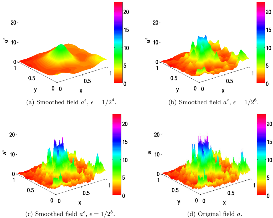
Figure 1: Three different regularizations of the same realization of a . \nu = 0.5 , L_c = 0.5 , \sigma = 1 .
