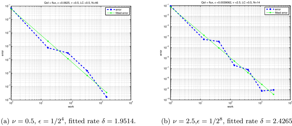
Figure 4: SC error computed as \mathbb{E}[Q_{h_l}^{\epsilon, SC} - Q_{h_L}^{\epsilon, SC}]^2 . L_C = 0.5 , \sigma = 1 .
