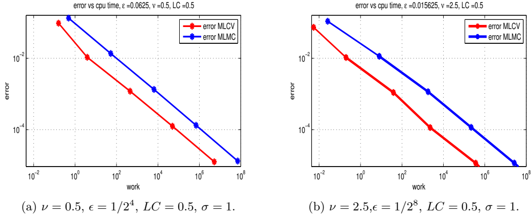
Figure 6: Error vs Computational cost. Error = SC error + Statistical error.
