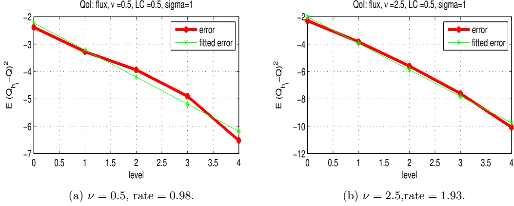
Figure 5: Discretization error computed as \mathbb{E}[Q_{h_i} - Q_{h_L}]^2 . LC = 0.5 , \sigma = 1 .
