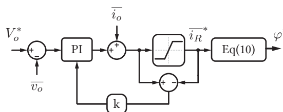
Fig. 4: Output voltage control implementation.
