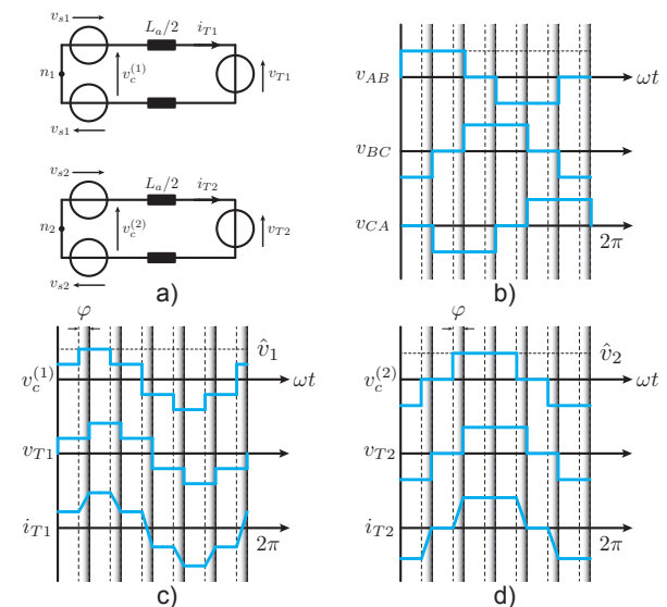
Fig. 3: a) Equivalent circuits of two MMCs connected to T_1 and T_2 , respectively b) Line voltages created by the SSC at converter's LV side c) Waveforms relevant for T_1 power flow analysis d) Waveforms relevant for T_2 power flow analysis.
