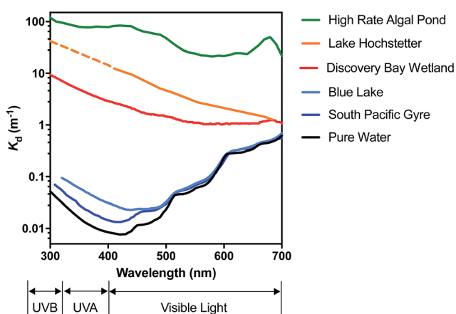
Fig. 3 Spectral irradiance attenuation in contrasting waters: pure water, the clearest known seawater on earth (S. Pacific Gyre near Easter Island 14 ), a clear lake water (Blue Lake, NZ (ref. 15)), a humic-stained lake (Lake Hochstetter, NZ; 16 UV data are extrapolated), a constructed wetland for polishing wastewater (Discover Bay wetland, CA 17 ); and a 'super-eutrophic' water laden with phytoplankton (a high-rate algal pond treating wastewater 18 ).
