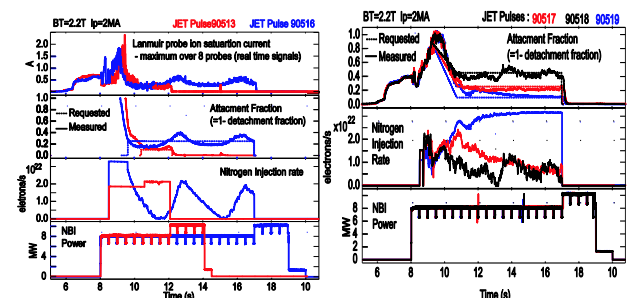
Fig.5 Closed loop detachment control without a) and with b) compensation for the non-linearity seen in figure 4.
