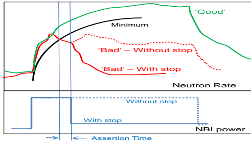
Fig.2 'Dud' detection. When the neutron is deemed unsatisfactory, the pulse is terminated.
