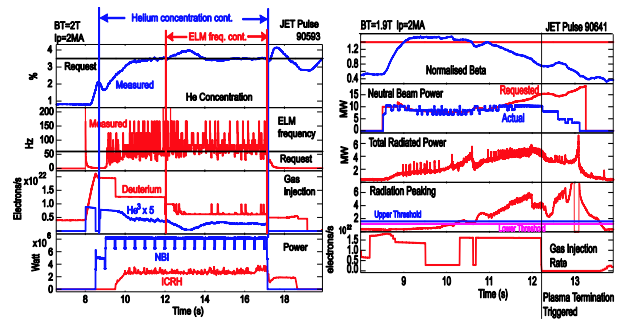
Fig.7 a) simultaneous control of the ELM frequency and He 3 concentration by injection of Deuterium and He 3 gas. b) simultaneous operation of a normalised beta controller by NBI and a bang/bang control scheme aimed at reacting to radiation peaking. At 12.2 seconds a discharge termination is triggered due to the detection of MHD activity.
