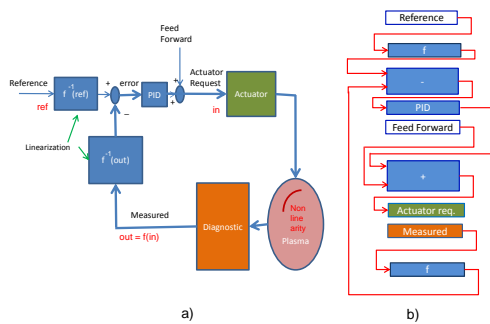
Fig.1 a) A simple closed loop algorithm with compensation for static nonlinearity. b) Schematic illustration of the implementation of this controller in the RTCC language.
