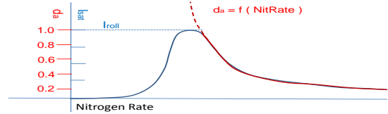
Fig.4 Sketch showing attachment fraction = I_{sat}/I_{roll} as a function of input gas flow rate.
