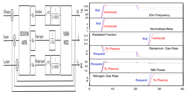
Fig. 8 a) 3x3 control block diagram b) Simulation of 3x3 control
