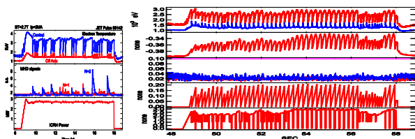
Fig.3 'a) Constant ICRH power. Long sawteeth trigger N=2 NTMs. ( 90142); b) Effective sawtooth pacing leading to the avoidance of NTMs.
