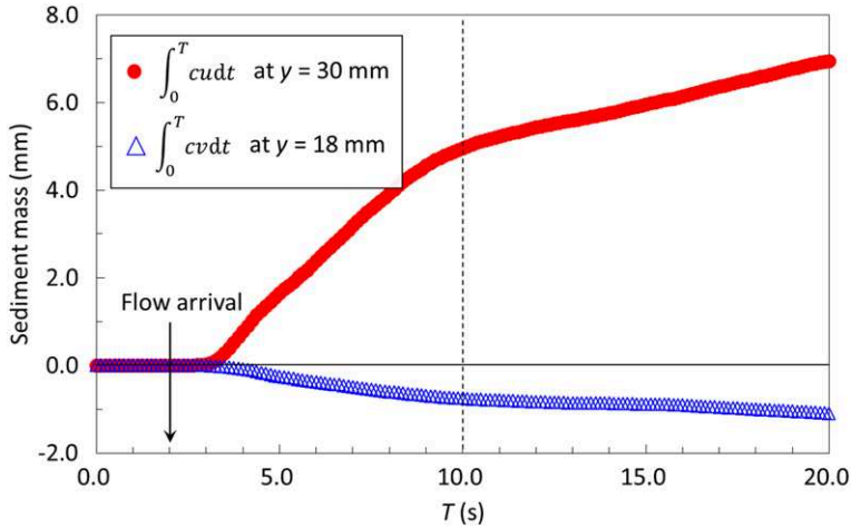
Fig. 10. Time-integrated sediment mass flux for u and v at y = 30 and 18 mm.
