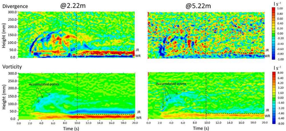
Fig. 4. Spatial and temporal divergence (upper part of the figure) and vorticity (lower part of the figure) distribution at x = 2.22 (left) and 5.22 m (right). Vertical and horizontal dashed lines represent the boundary of the head and body, and the horizontal velocity maximum.
