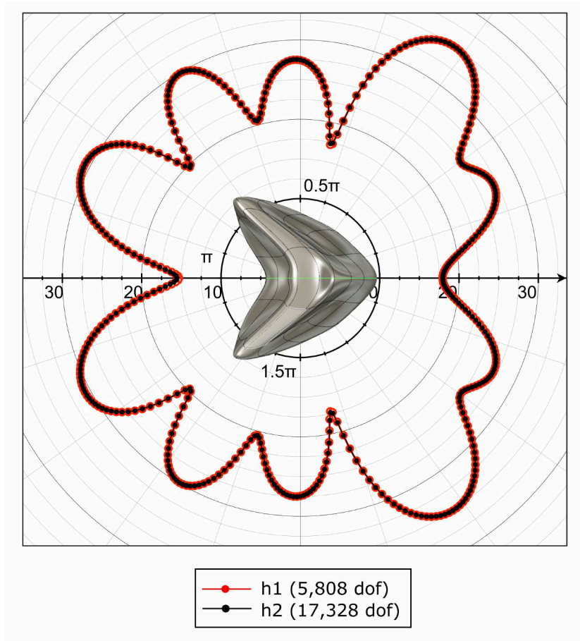
Figure 31: The computed radar cross section profile for the concept model illustrated in Figure 29 with a normalized wavenumber ka = 9.31 .
