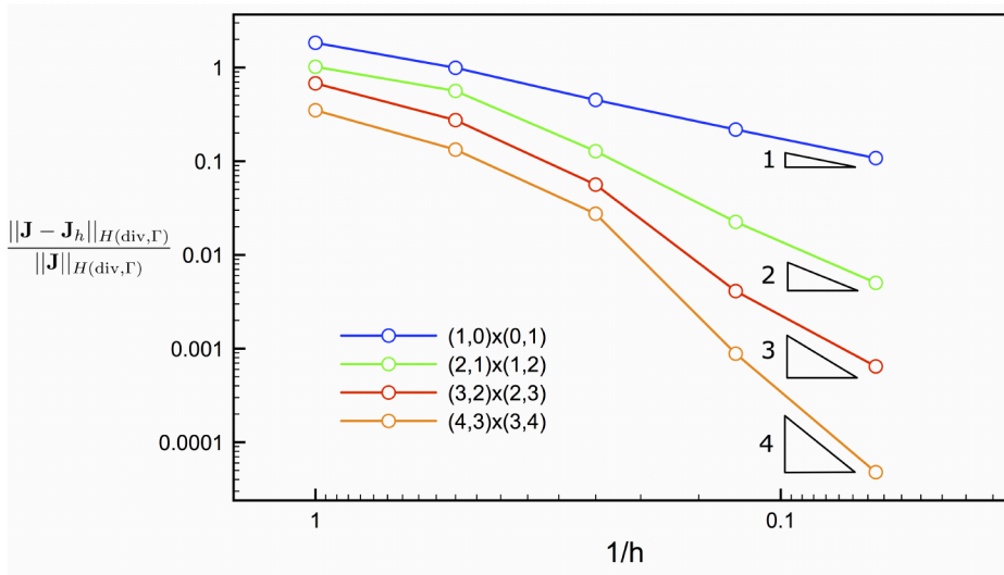
Figure 16: Mie scattering convergence study with k = 3 : relative error norms for B-spline discretizations and theoretical convergence rates.
