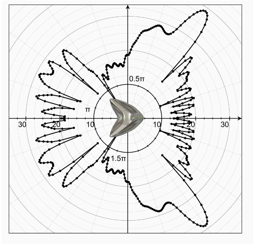
Figure 33: The computed radar cross section profile for the concept model illustrated in Figure 29 with a normalized wavenumber ka = 46.55 .
