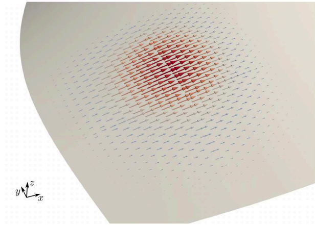
(a) \mathbf{N}_{19}^{\text{div}}(\mathbf{x})
