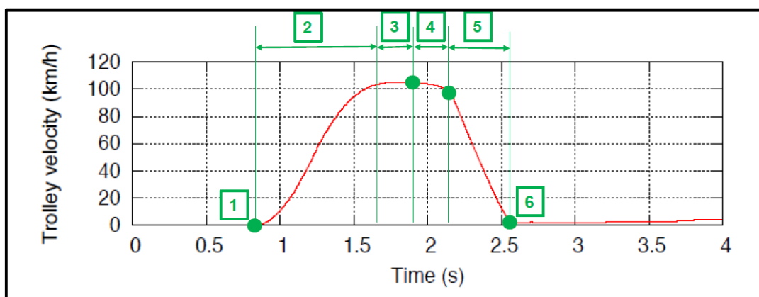
Figure 5: Phases of each ditching test run
