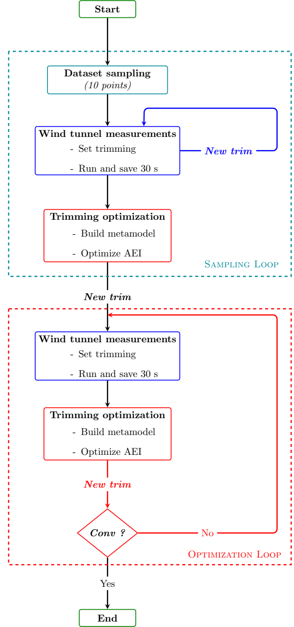
Figure 4: Trimming optimization procedure.
