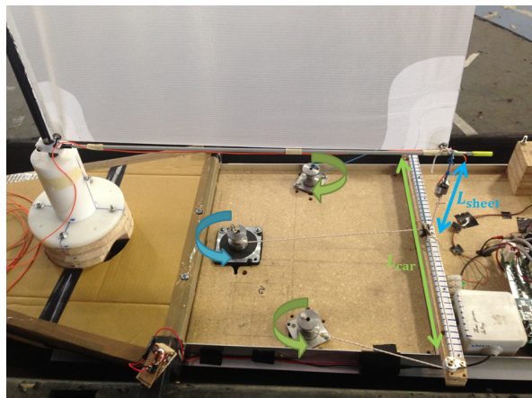
(b) Close view on the trimming system.
