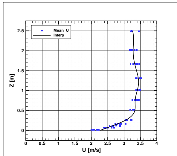
Figure 11: Inflow velocity profile.
