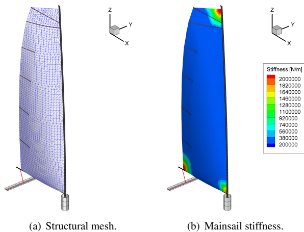
Figure 9: Numerical model of the sail.
