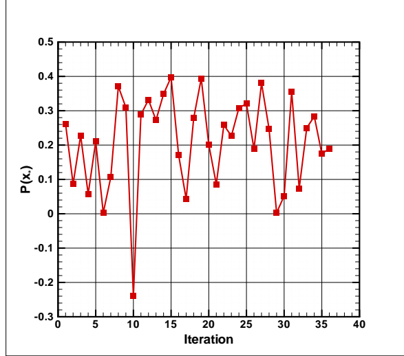
Figure 6: Experimental measurements of the performance for the sequence of proposed optima. Case of \sigma_\epsilon = 0 .
