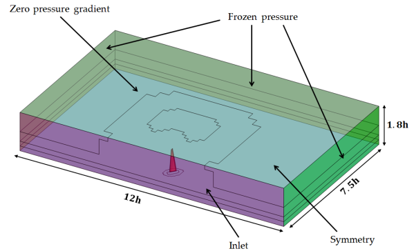
Figure 10: Boundary conditions for the flow solver.
