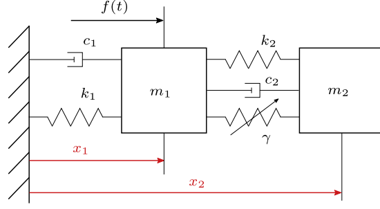
Fig. 1. Duffing-like system.
