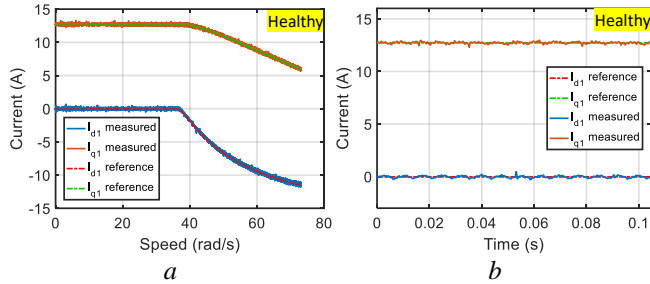
Fig. 6. (Experimental results) Currents in (d_1-q_1) frame in healthy mode (a) Currents vs speed, (b) Currents vs time at 20 rad/s
